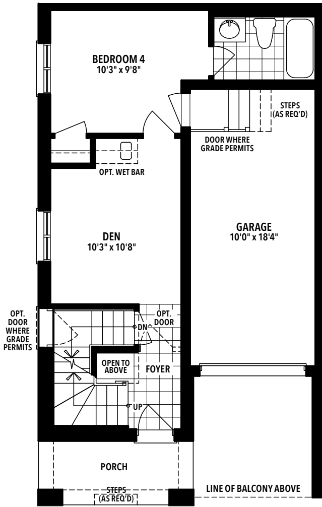
LOWER FLOOR PLAN ELEV. B & C
