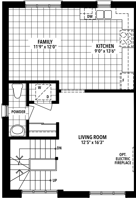
MAIN FLOOR PLAN ELEV. A
