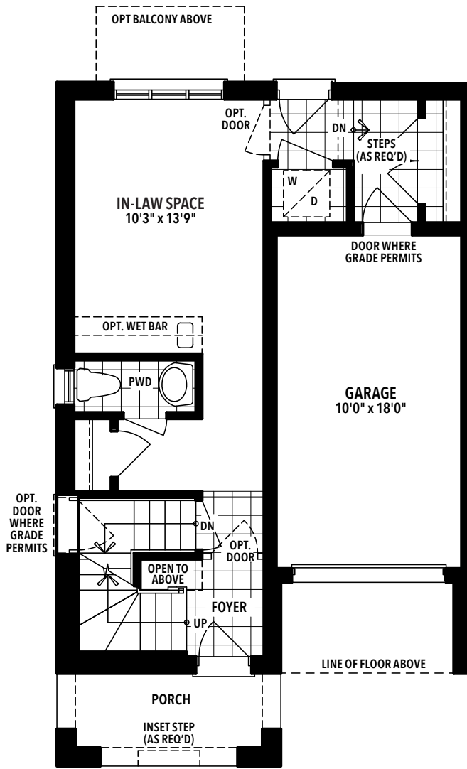
LOWER FLOOR PLAN ELEV. A
